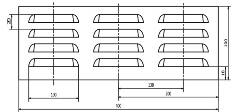
Top Elevation - 100mm x 400mm
